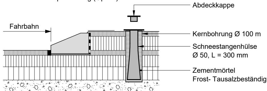
Bodenhülse in Asphalt Belag (Option)
